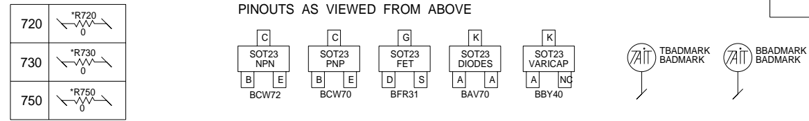
PINOUTS AS VIEWED FROM ABOVE
